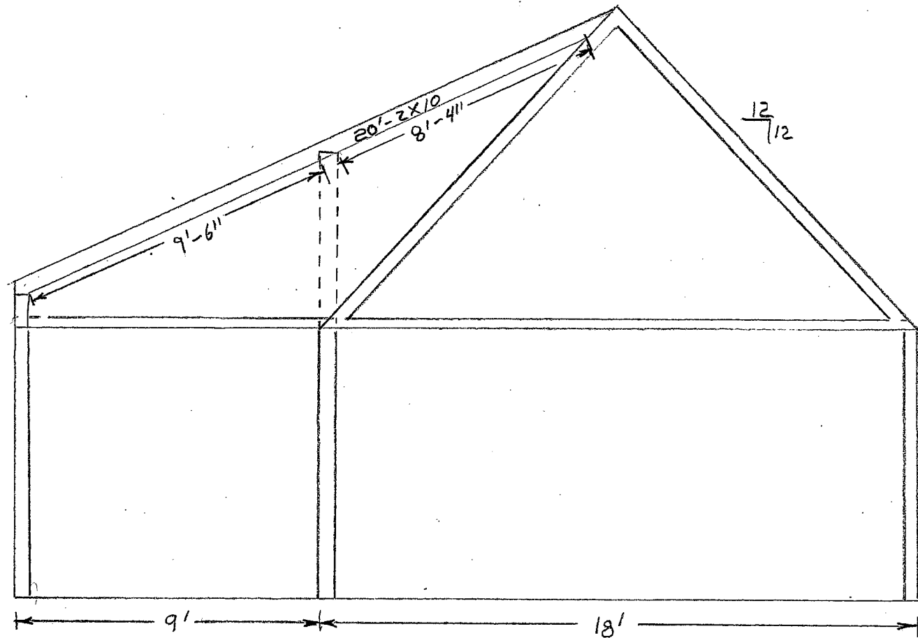
CORRECTED FRAMING DETAIL - CROSS SECTION
