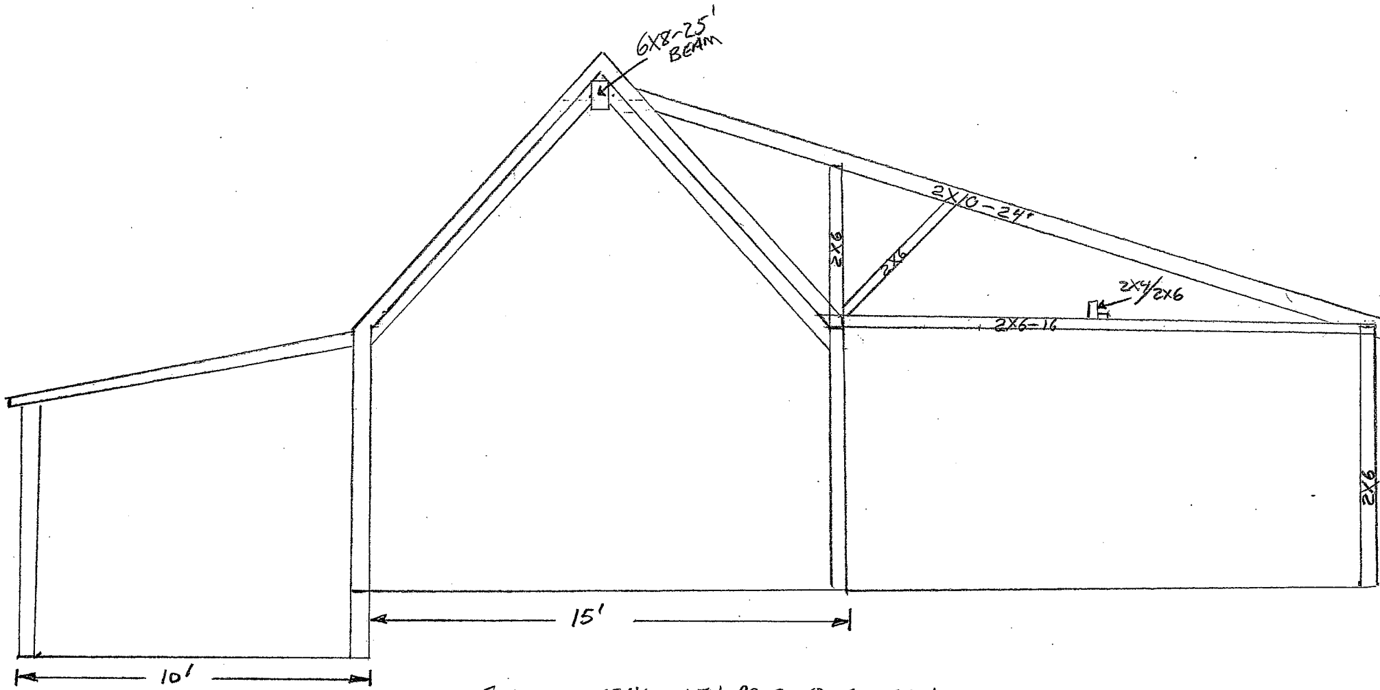
FRAMING DETAIL WITH PROPOSED ADDITION
