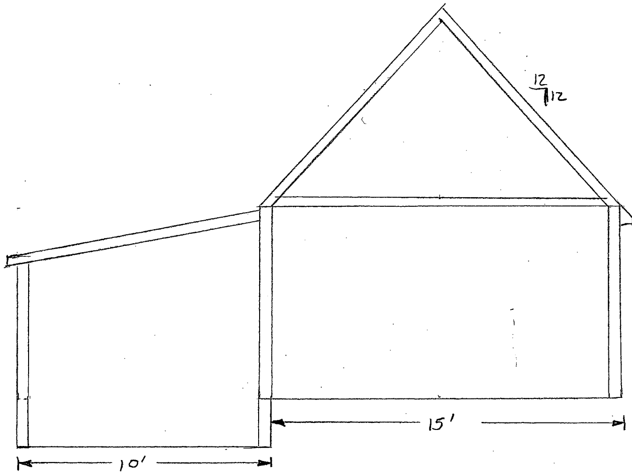
EXISTING FRAMING DETAIL - CROSS SECTION
