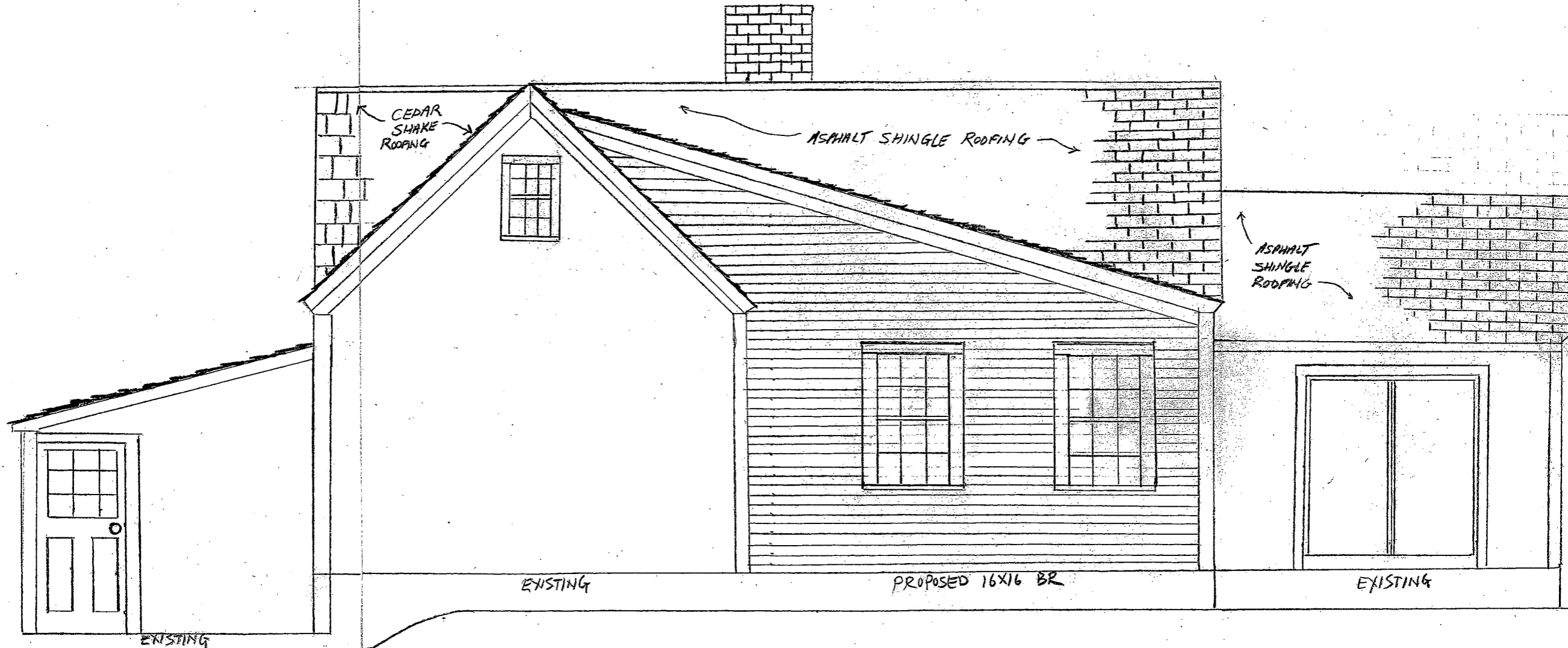
REAR VIEW - NORTH
