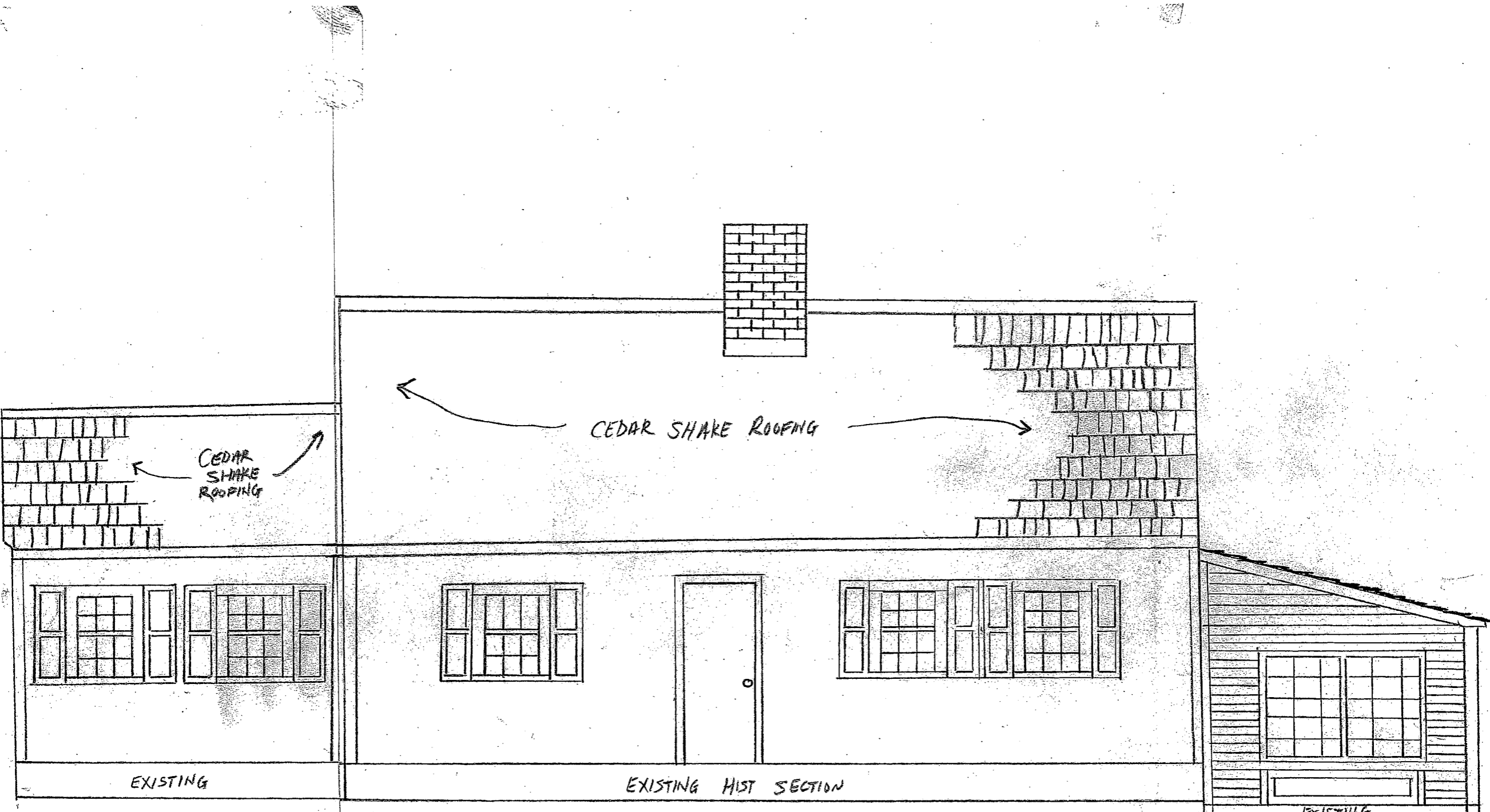
FRONT VIEW - SOUTH
