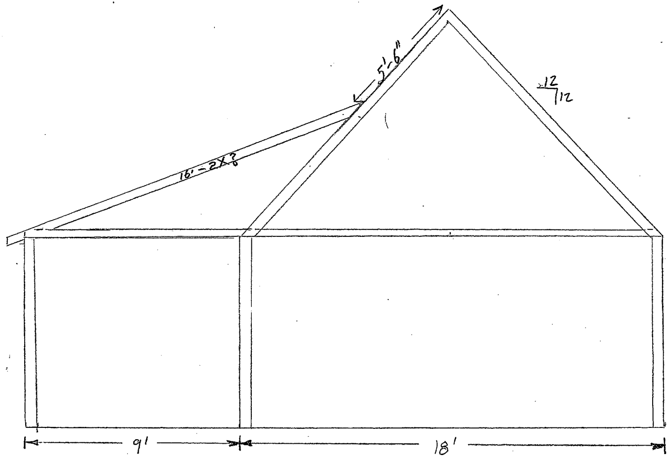
EXISTING FRAMING DETAIL - CROSS SECTION
