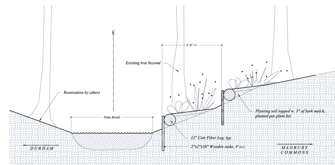
Petite Brook Rehabilitation Shore Stabilization Detail
