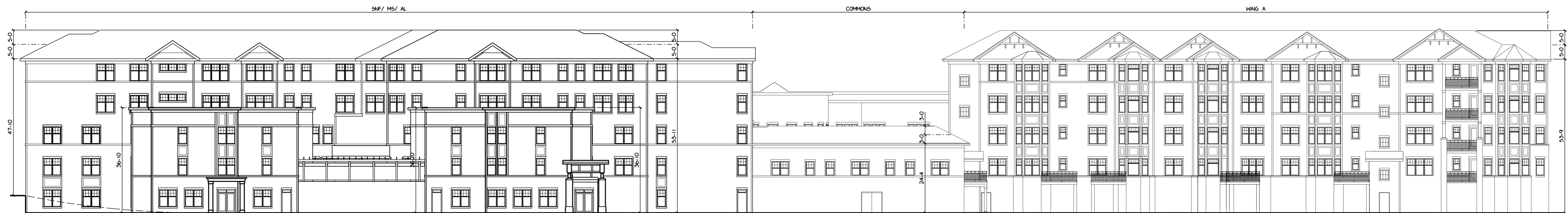
ELEVATION (DPW LAND) 3 1/16" = 1'-0"
