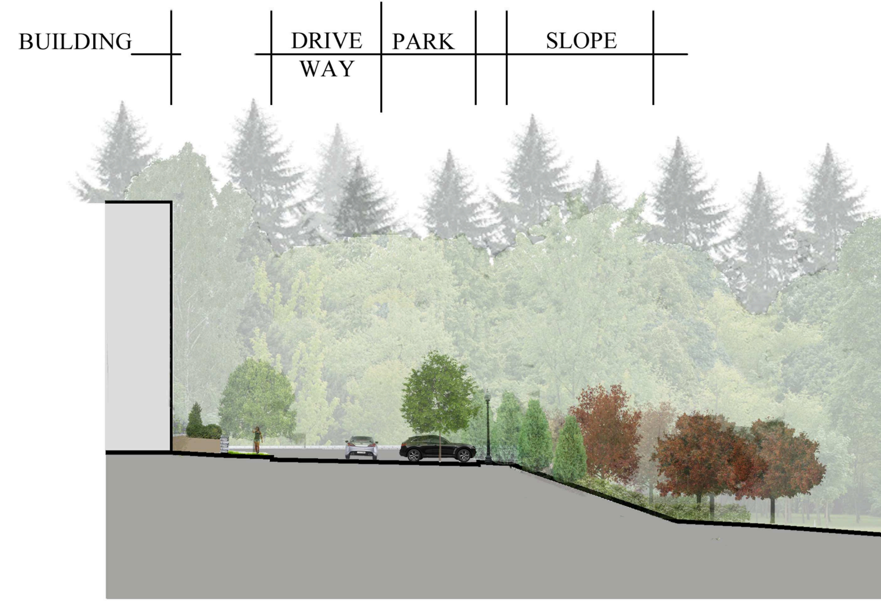
Section E-E' 0 5 10 20 40
