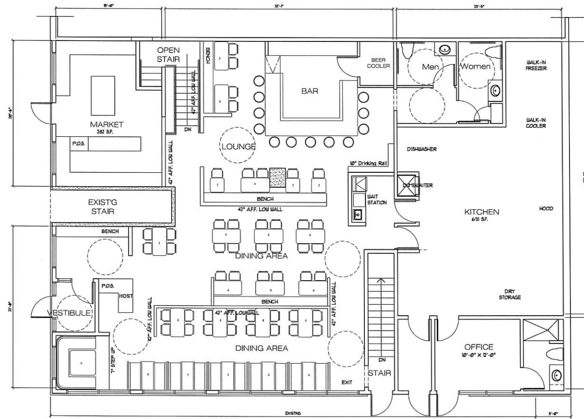
1 Main Level Floor Plan 1/4" = 1'-0"
