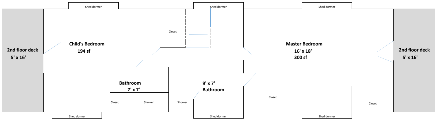
Proposed Second floor 16' x 42' 696 sf 5088 cu ft
